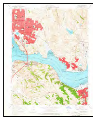
Benicia 1959 7.5-minute, 24000 Aerial Photo Revised 1958
