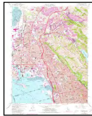
Richmond 1980 7.5-minute, 24000 Aerial Photo Revised 1979
