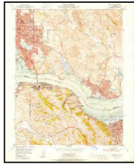
Benicia 1952 7.5-minute, 24000 Aerial Photo Revised 1948
