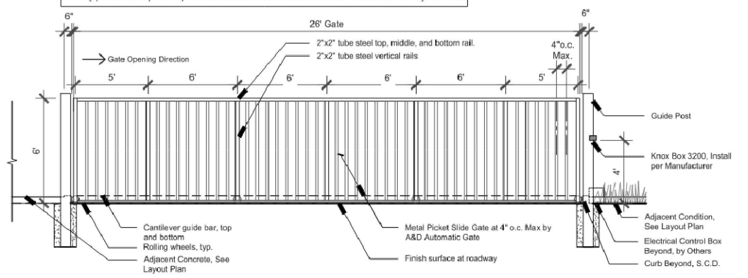
METAL PICKET VEHICULAR SLIDING GATE NOT TO SCALE
